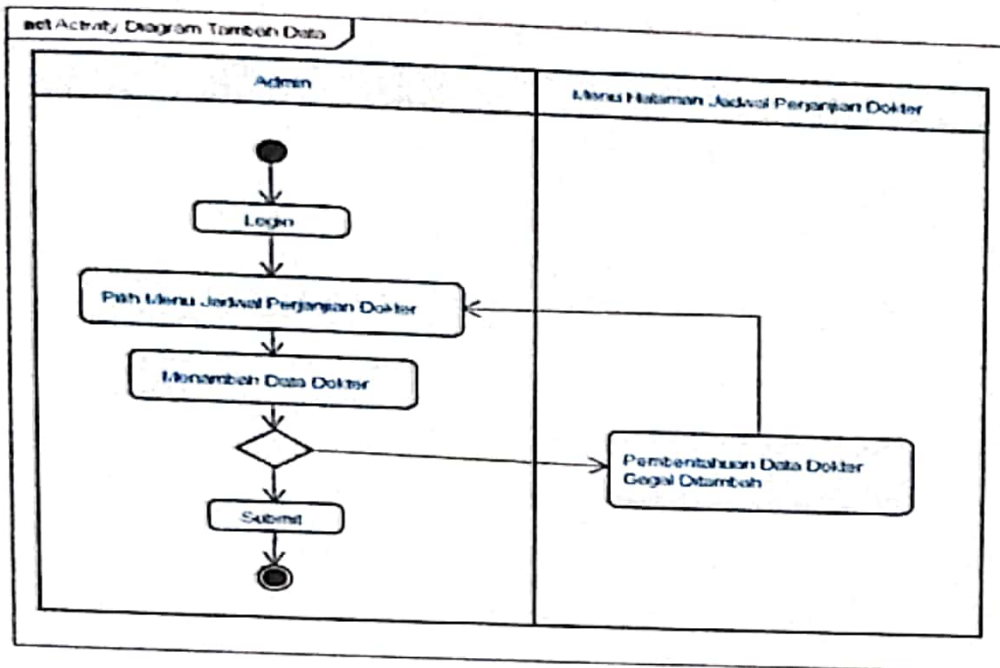
Gambar 5.3 Activity Diagram Tambah Data Dokter
