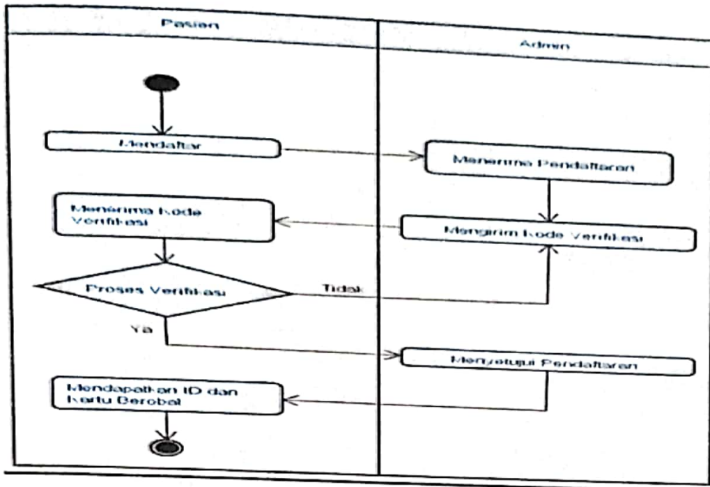
Gambar 5.1 Activity Diagram Pendaftaran
