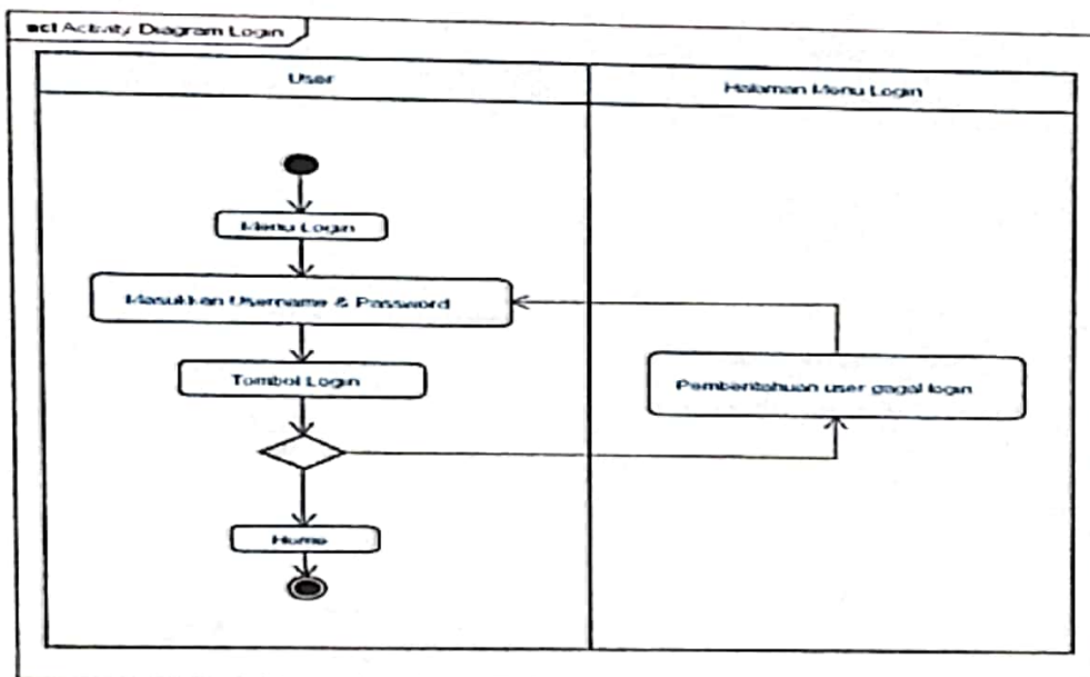
Gambar 5.2 Activity Diagram Login
