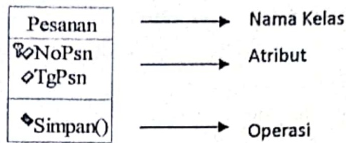
Class Diagram
